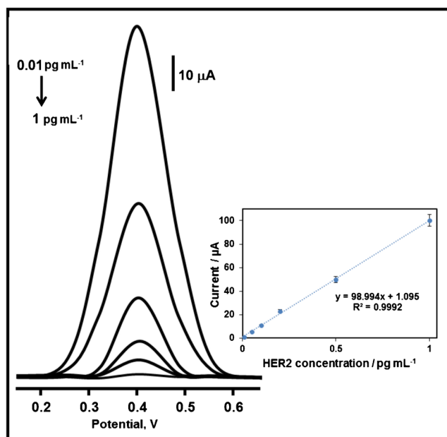
Fig. 4 Concentration effect (from 0.01 to 1.0 pg mL -1 HER2) on immunosensor signals, Inset: Calibration curve for voltammetric HER2 immunosensor (Potential range is 0.0/+0.6 V; Parameters are frequency of 50 Hz, pulse amplitude of 20 mV and scan increment of 3 mV)
