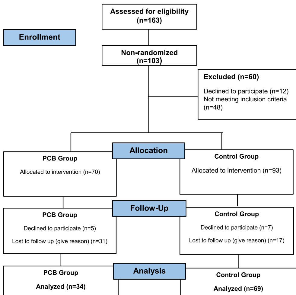
FIGURE 1 | CONSORT diagram.
