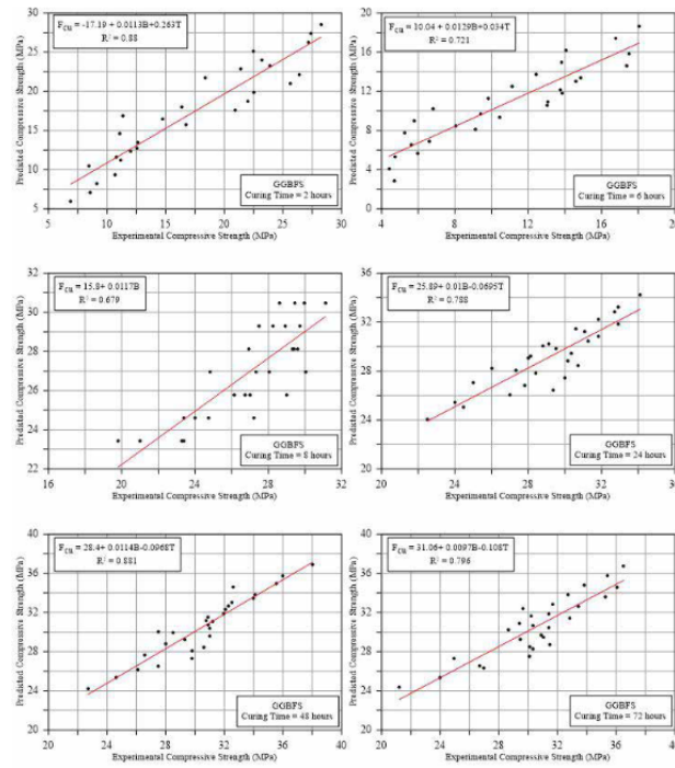
Figure 3. Step-wise formula of compressive strength versus GGBFS binder content and curing temperature for different curing times
