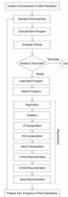
Figure 1. Flowchart of GEP
