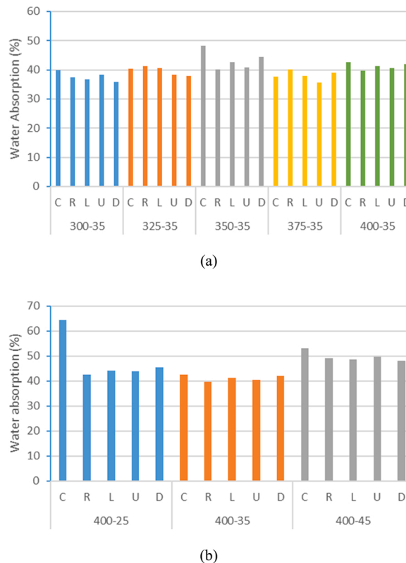
Fig. 14. Water absorption's variation of SC according to, (a) pressure injections, (b) jet grout's rotations.
