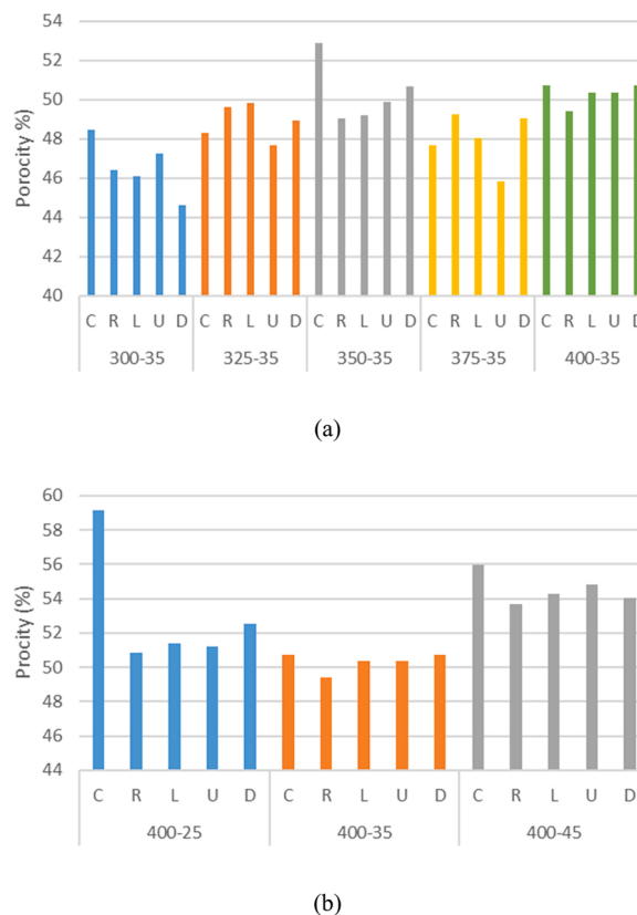
Fig. 15. Porosity variation of SC according to, (a) pressure injections, (b) jet grout's rotations.
