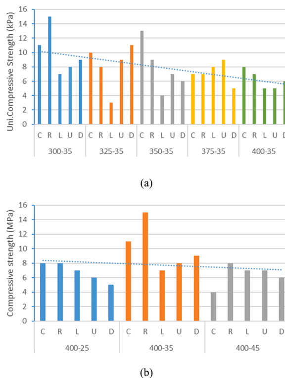
Fig. 10. Compressive strength variation of SC according to, (a) pressure injection, (b) jet grout's rotations.
