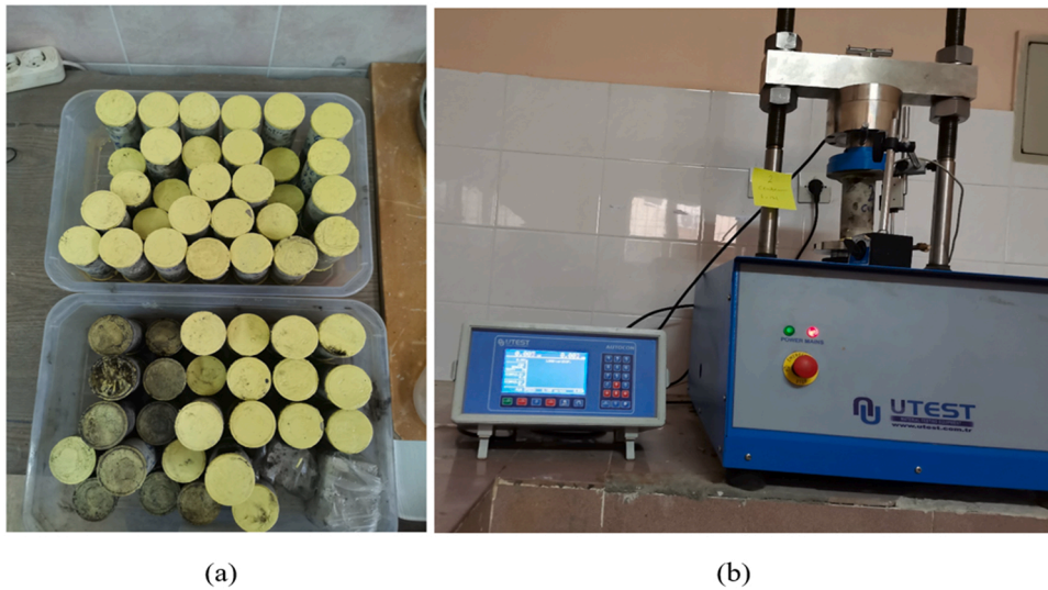
Fig. 7. Test specimens of SC, (a) covering the samples, (b) Unconfined compression machine.
