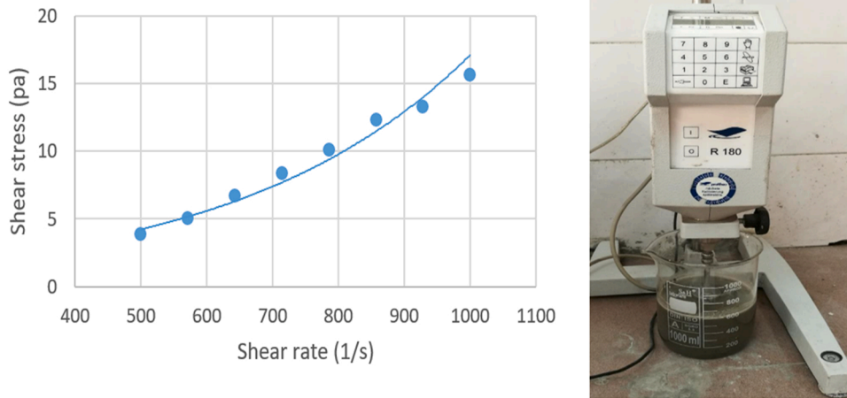
Fig. 3. Rheological properties of jet grout column: (a) Shear stress versus shear rate relationship; (b) Coaxial rotating cylinder Rheometer.
