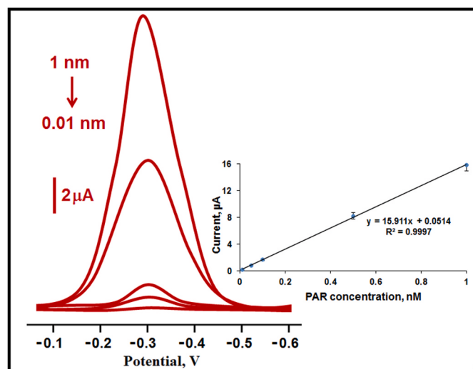
Fig. 5. DPVs with different PAR concentrations at MIP/ \text{MoS}_2\text{NPs}@MWCNTs /GCE in PBS with pH = 7.0 (in a concentration range of 0.01–1.0 nM). Inset: PAR's calibration curve.
